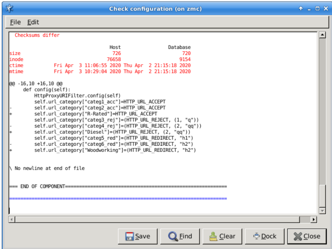
Figure 7. Validating configuration
