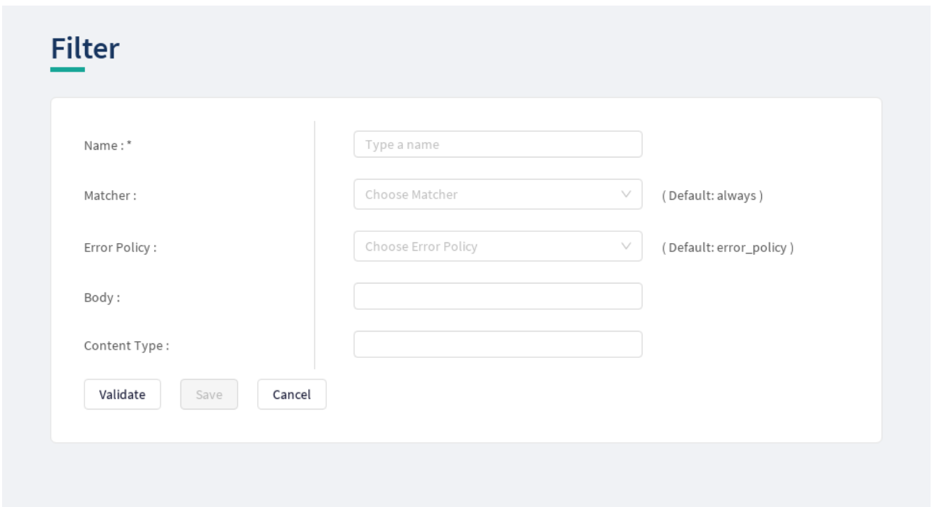
Figure 29. Configuring a filter plugin in the Web User Interface
