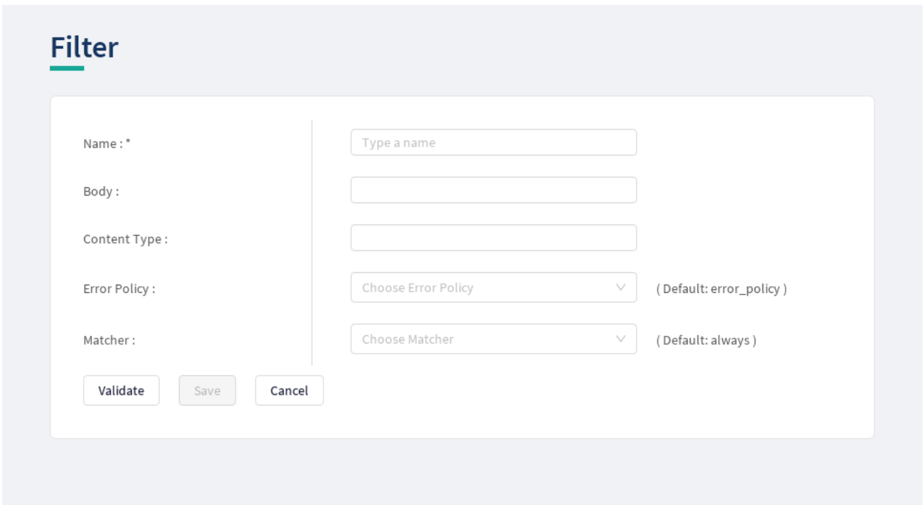
Figure 50. Configuring a filter plugin in the Web User Interface
