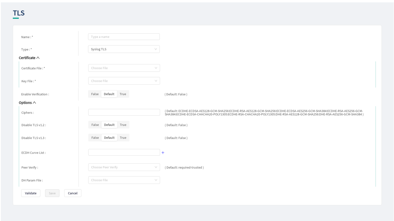
Figure 43. Configuring Syslog TLS in the Web User Interface
